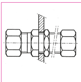
Union passe-cloison
